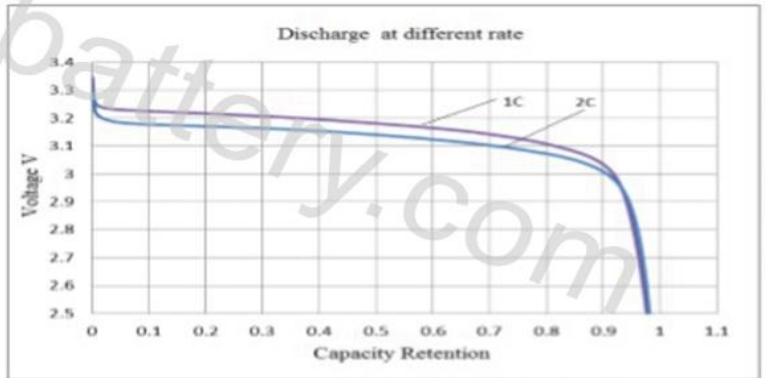
A typical curve of single cell discharged at room temperature
